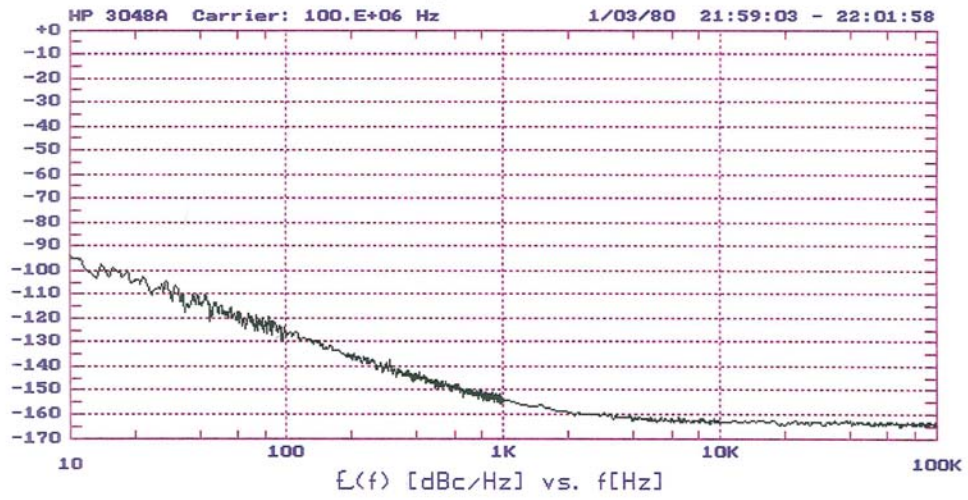
Figure 2 SSB Phase Noise of Crystal Reference Oscillator
