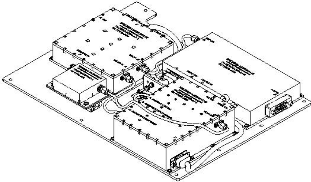
Figure 3 Mechanical Configuration
