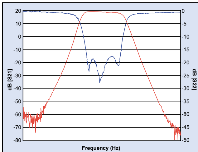
Fig. 4. The switch filter bank's typical transfer function and return loss.
