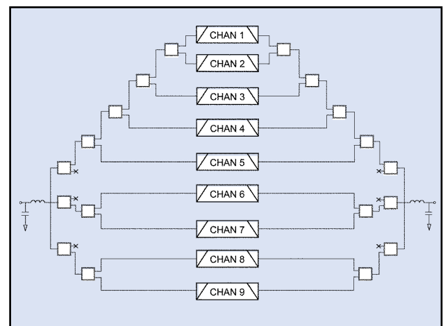
Fig. 2. The hybrid radial-binary tree configuration.
