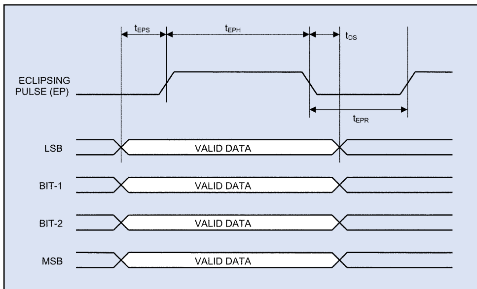
Fig. 3. Logic timing of the eclipsing pulse.
