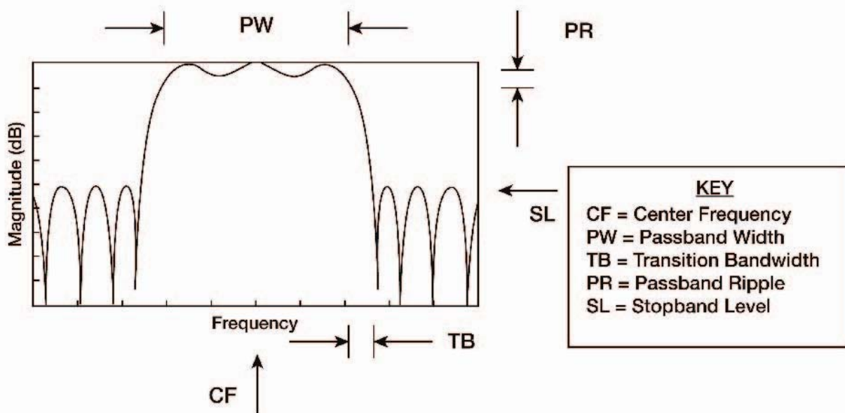
Figure 1: Characteristics of typical SAW filter
